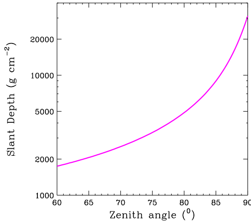
Figure 1. Slant depth for very inclined showers at the southern site of the Pierre Auger Observatory, ranging from 1740 \text{ g cm}^{-2} at 60^\circ zenith angle to 31,000 \text{ g cm}^{-2} at 90^\circ
